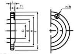
Dimension - Flange
