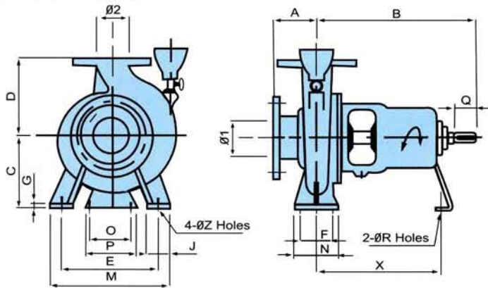
Dimension - Pump
